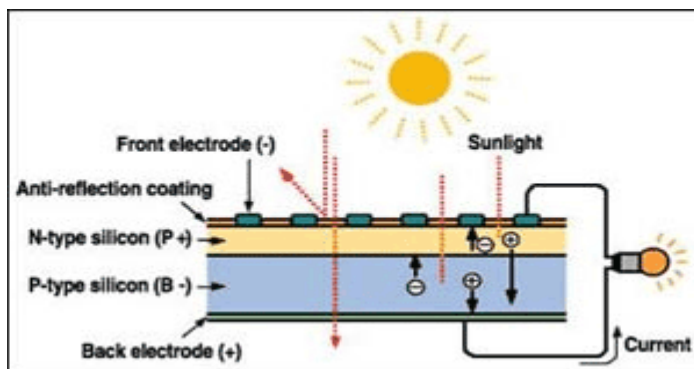
Fig4. Shows photovoltaic system
